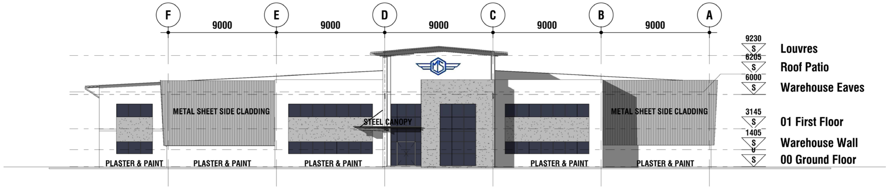
North Elevation
