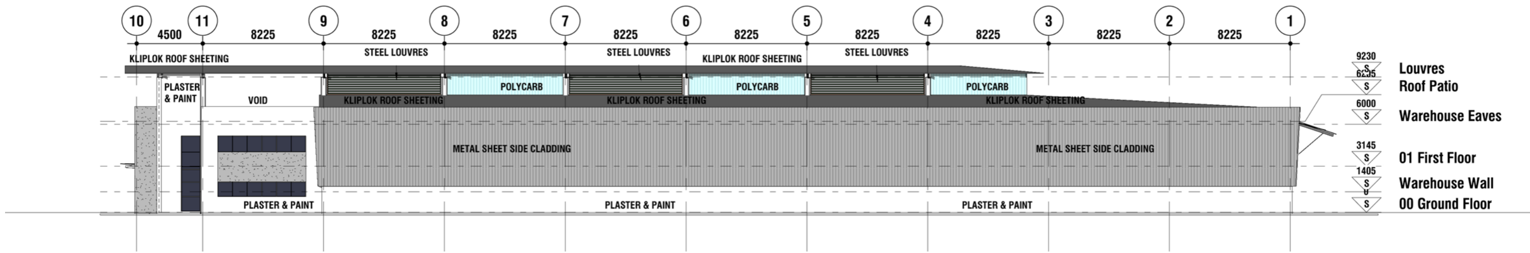
West Elevation
