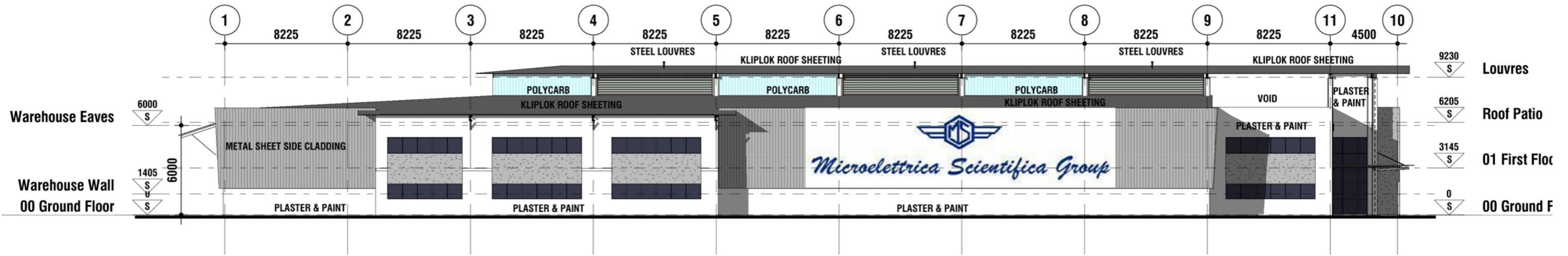
East Elevation
