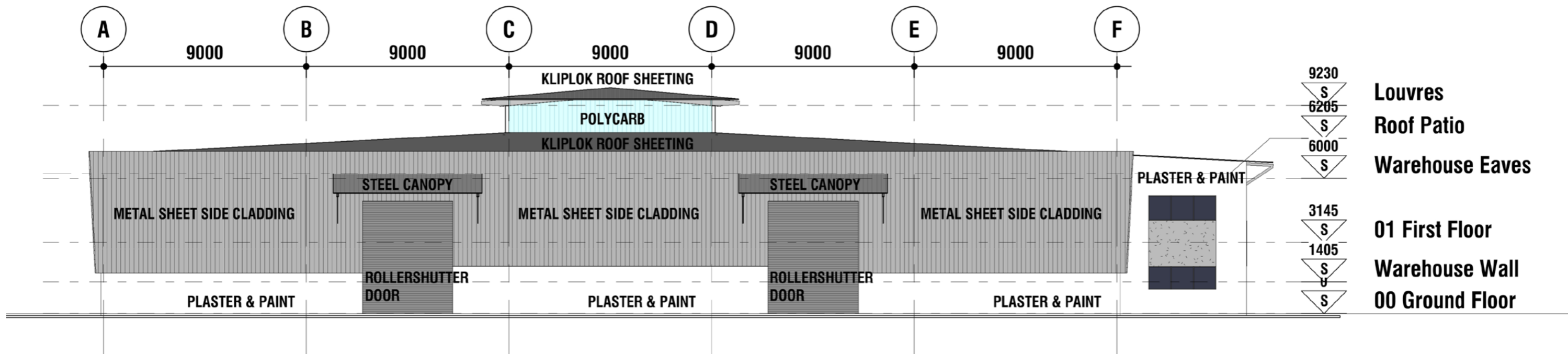
South Elevation
